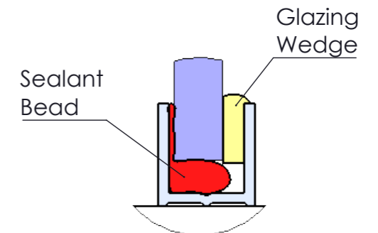
Glass Panel Silicone Detail
