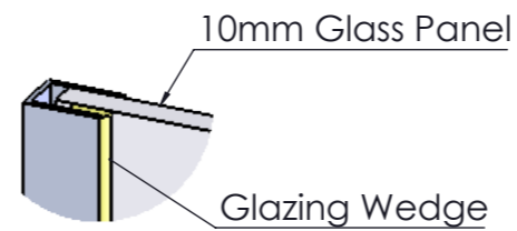
Glass To Wall Tolerance DETAIL A
