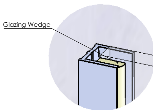
Glass To Wall Tolerance DETAIL A
