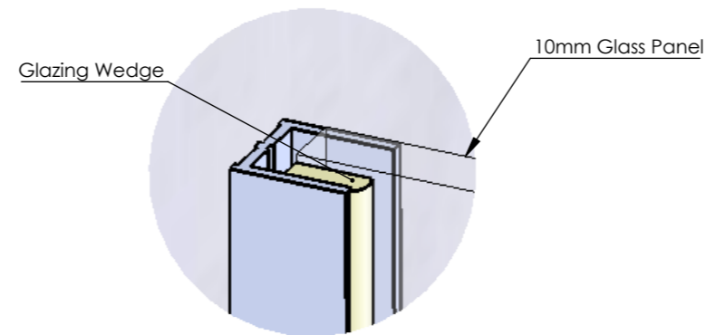
Glass To Wall Tolerance DETAIL A
