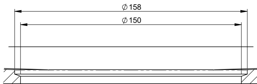
DETAIL B SCALE 2 : 3
