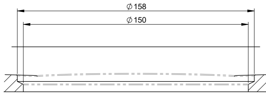
DETAIL B SCALE 2 : 3
