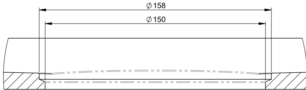
DETAIL B SCALE 2 : 3
